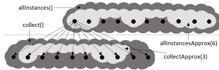
Fig. 4. Idea for Approximate Operators
