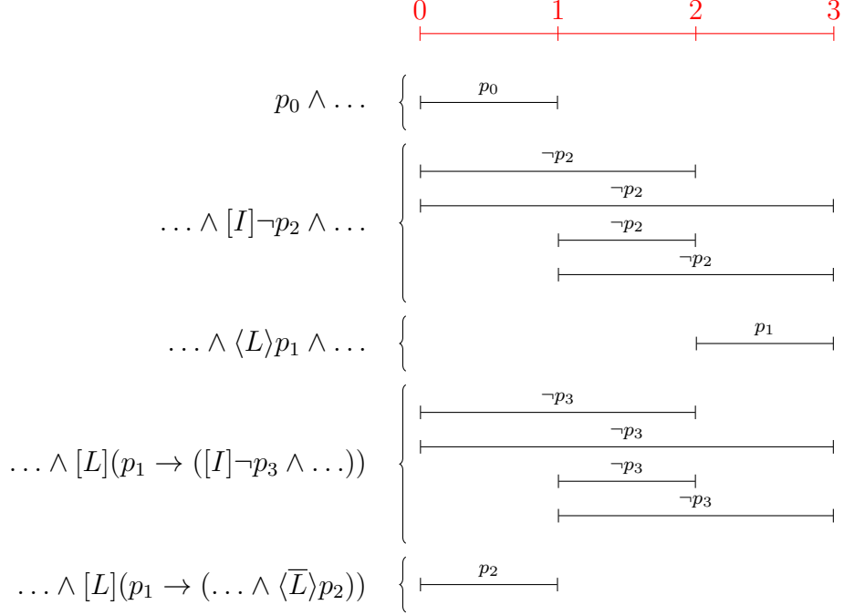
Figure 7: Example of a possible model for \varphi_1 from Table 3.
