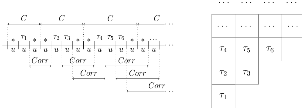
Figure 6: A model of \varphi_{\mathcal{T}} and its interpretation as a tiling of the second octant.
