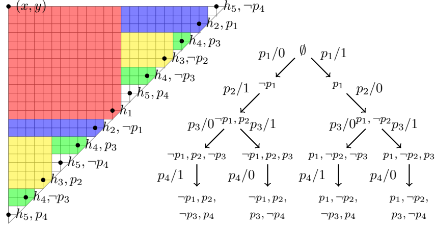
Figure 2: A tree-model for \theta = \forall p_1 \exists p_2 \forall p_3 \exists p_4 ((p_1 \vee p_2) \wedge (\neg p_1 \vee \neg p_2) \wedge (p_3 \vee p_4) \wedge (\neg p_3 \vee \neg p_4)) (right-hand side) and its embedding into a compass structure (left-hand side).
