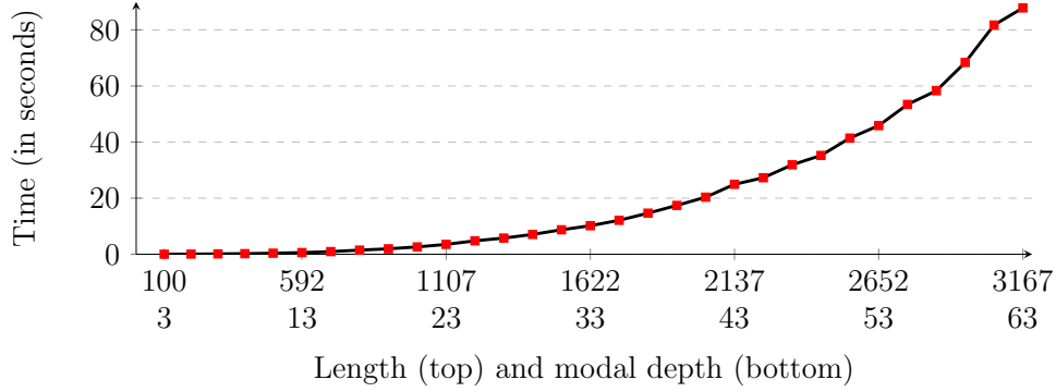
Figure 8: Elapsed time for satisfiable formulæ (by length and modal depth).
