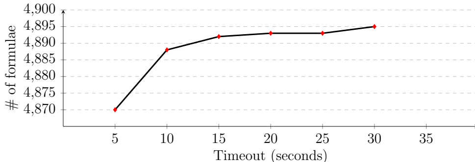
Figure 9: Timeouts versus number of finalized formulae.
