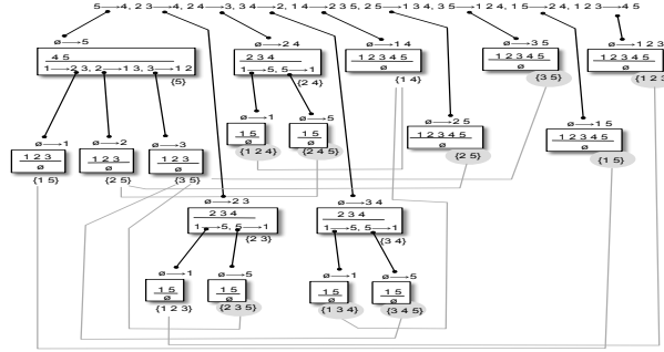
Fig. 2. \text{MinGen}_0 Execution
