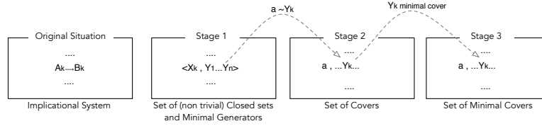
Fig. 1. Stages of D -basis algorithm
